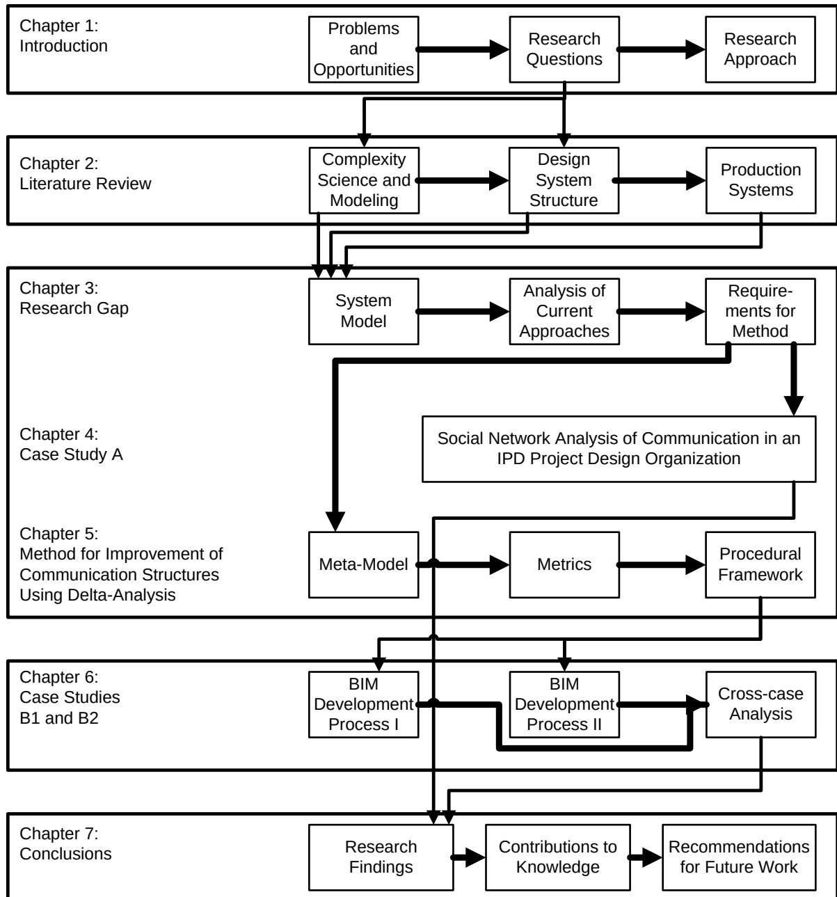
Figure 3: Dissertation Structure
