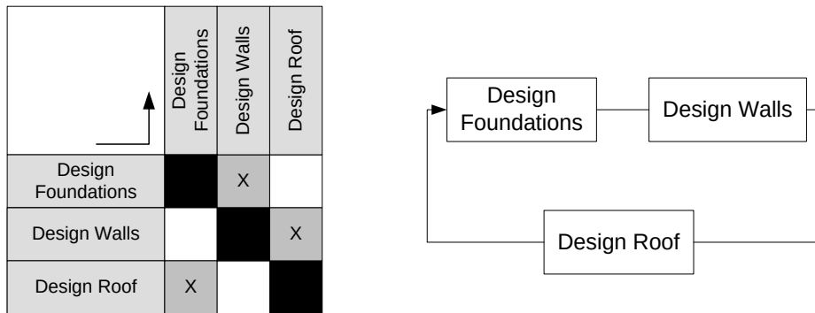
Figure 7: Binary DSM of a Simple Process
